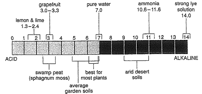
The pH scale and some commonly known substances
